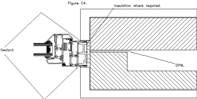
Flush reveal with external render for replacement windows/doorsets with frame shuffled into position
