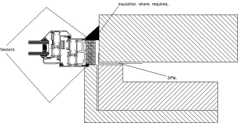
Frame forward of DPM
