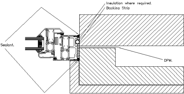
Flush reveal frame bridging DPM joint width from 6 mm to 15 mm
